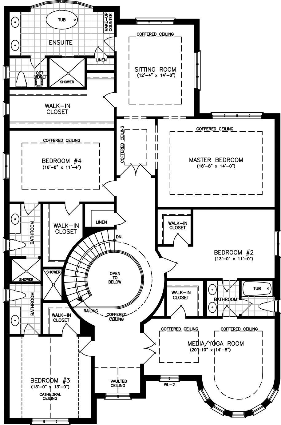
SECOND FLOOR
