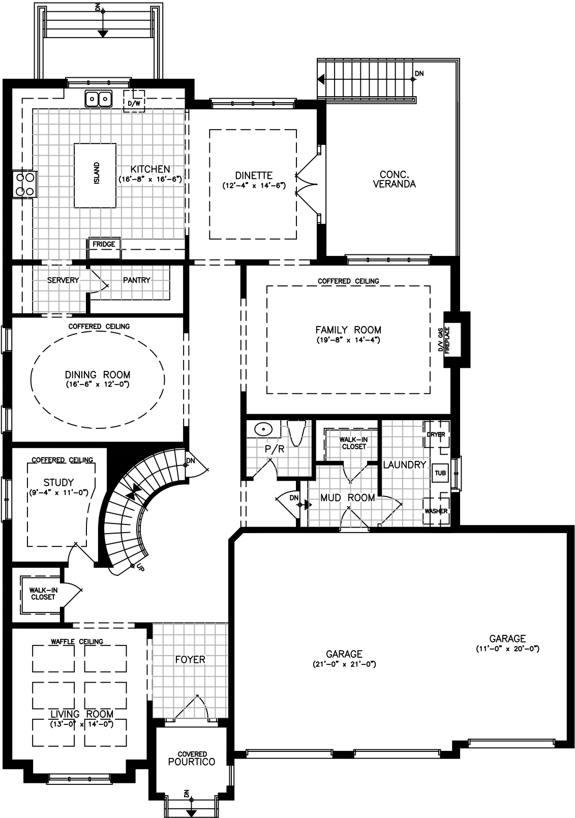
FIRST FLOOR
